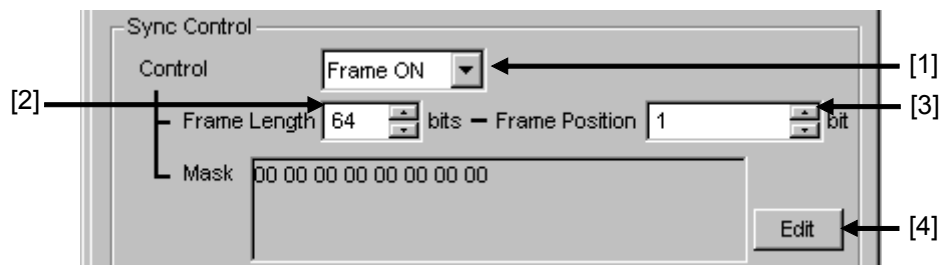
Figure 5.2.3-1 Synchronization establishment method setting items in Sync Control area
