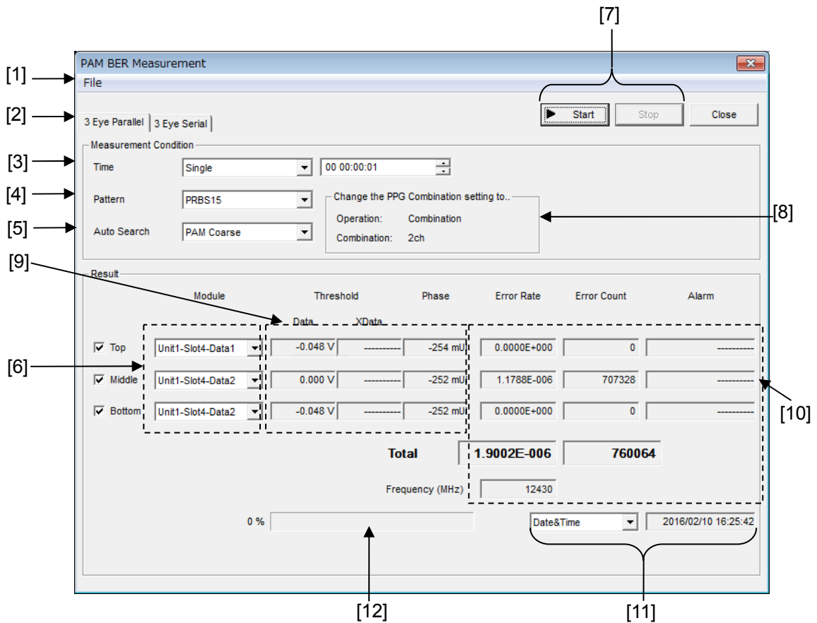
Figure 5.14.1-2 PAM BER Measurement window (3 Eye Paralle mode)
