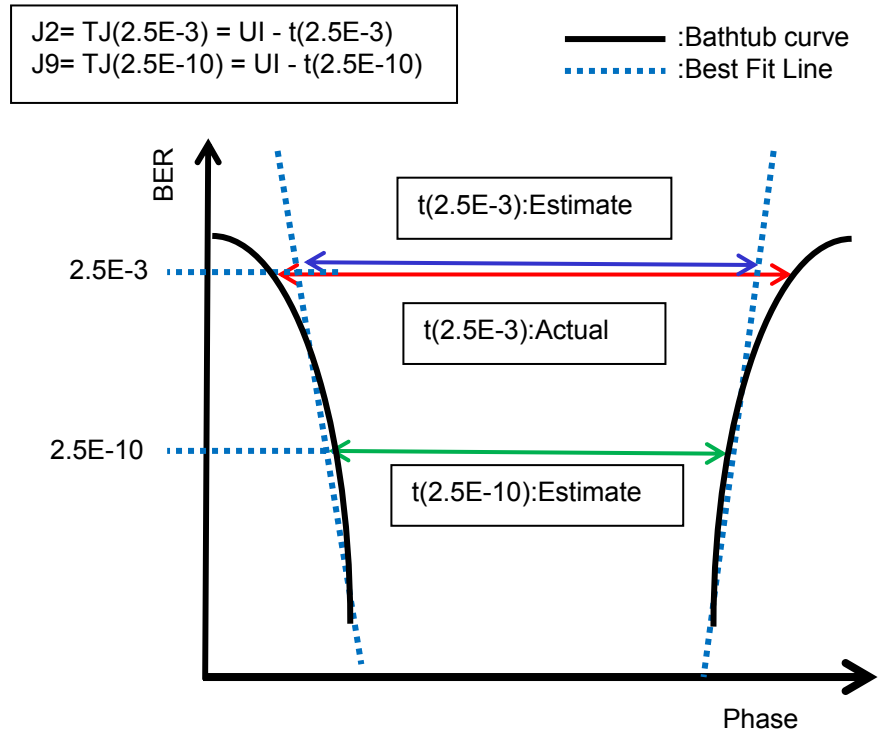
Figure 5.12.1.2-4 J2 Calculation
