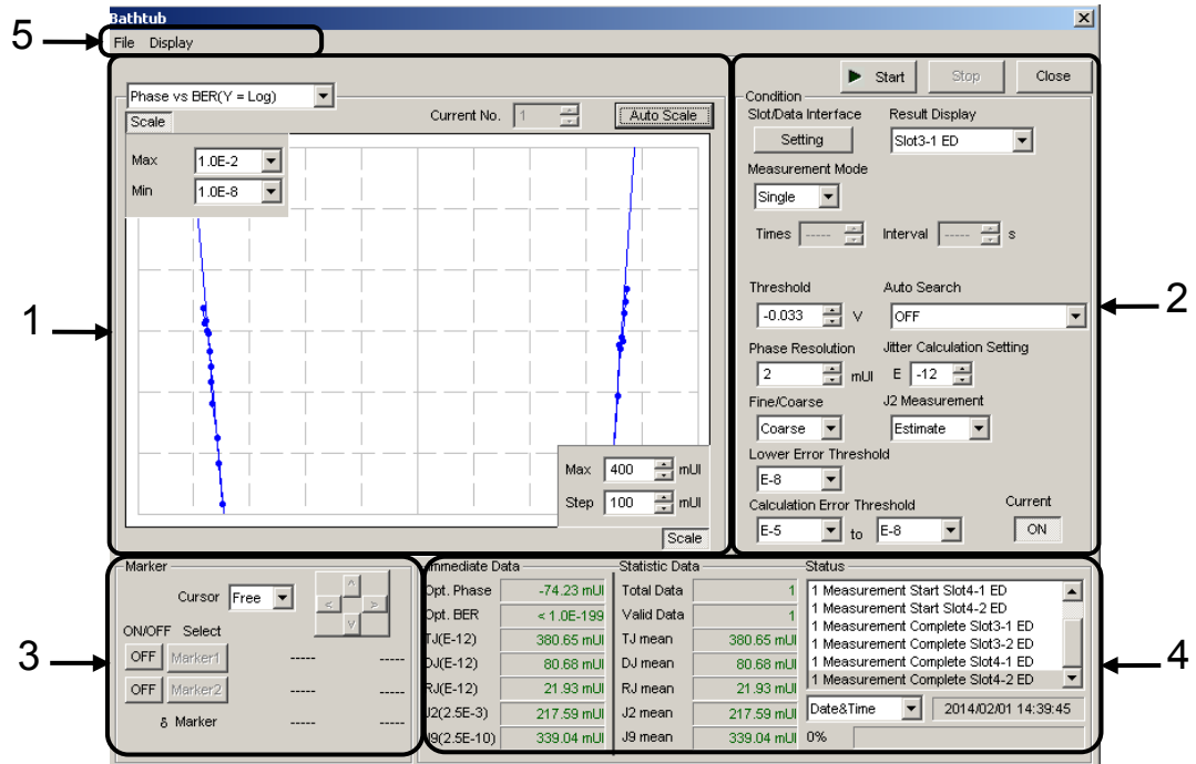
Figure 5.12.1-1 Bathtub window
