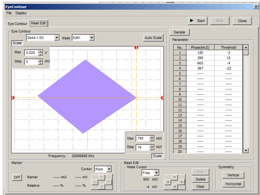
Figure 5.15.6-6 Mask Setting
