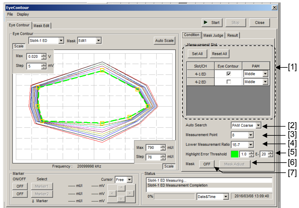
Figure 5.15.1-1 Eye Contour window
