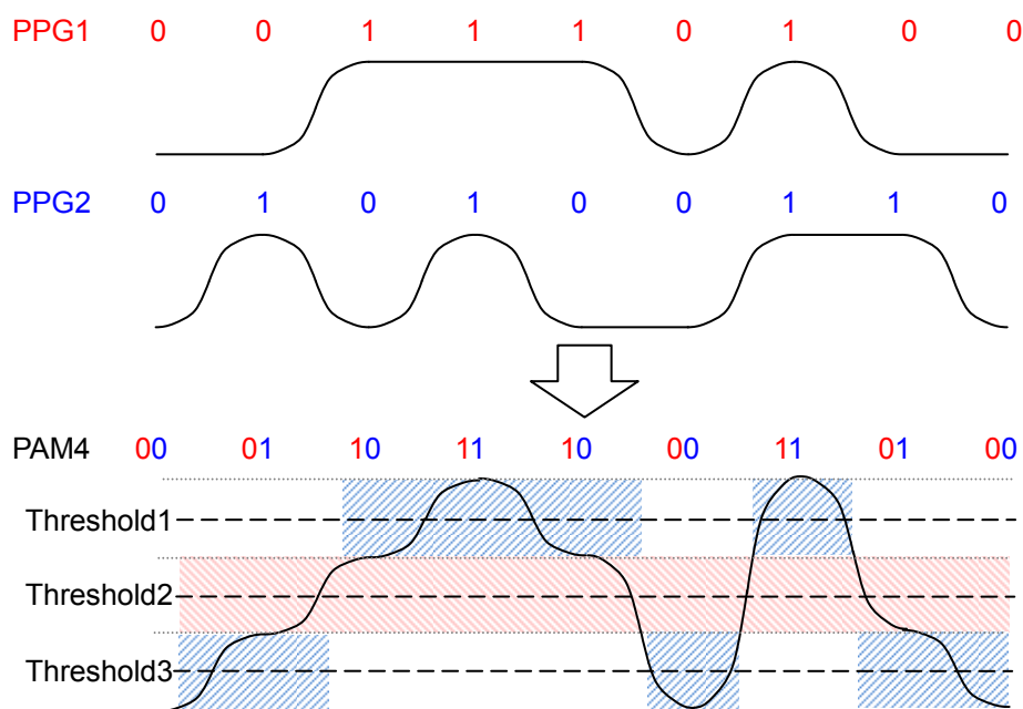
Figure F.1-2 PAM Signals and Thresholds at BER Measurement
