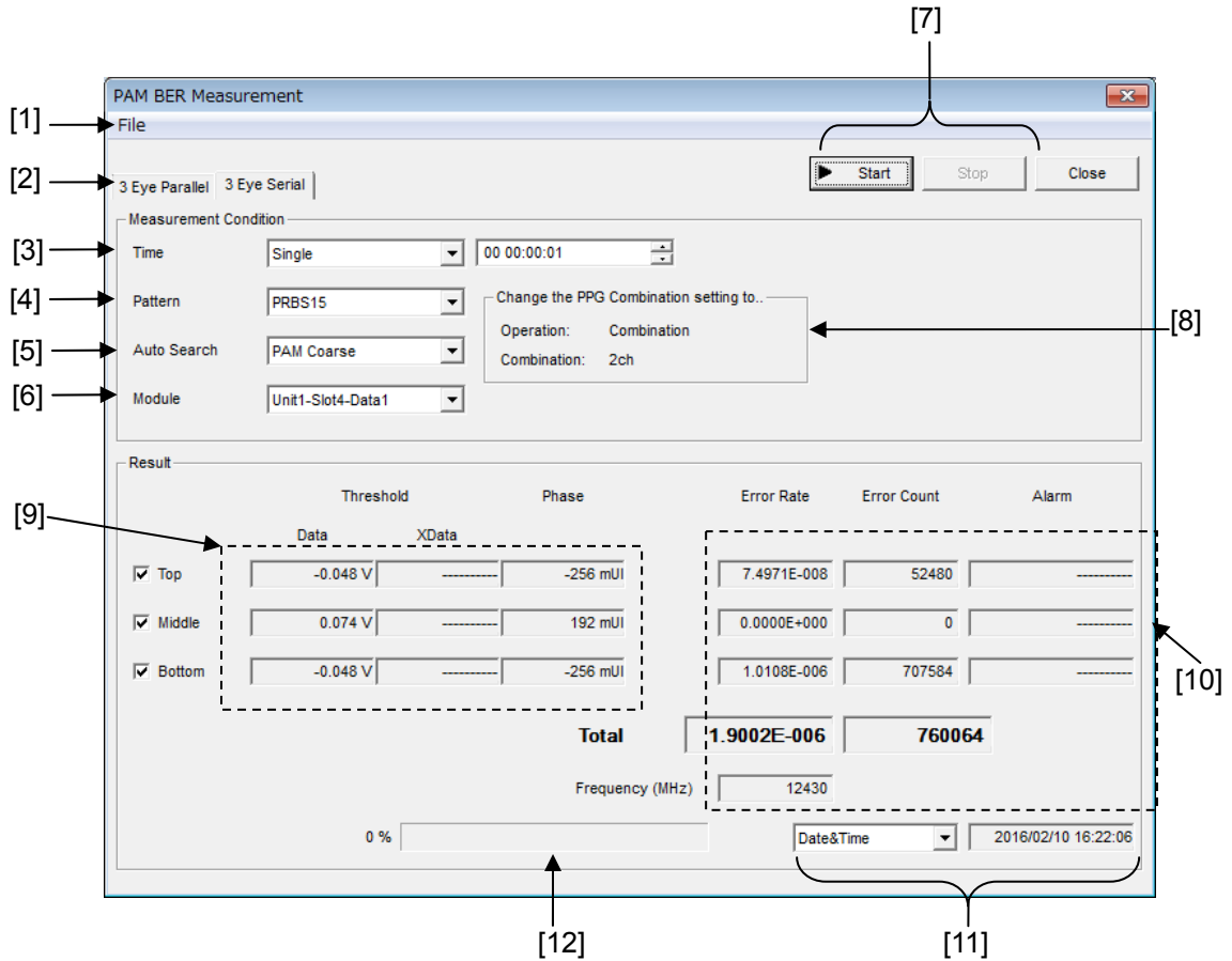
Figure 5.14.1-1 PAM BER Measurement window (3 Eye Serial mode)
