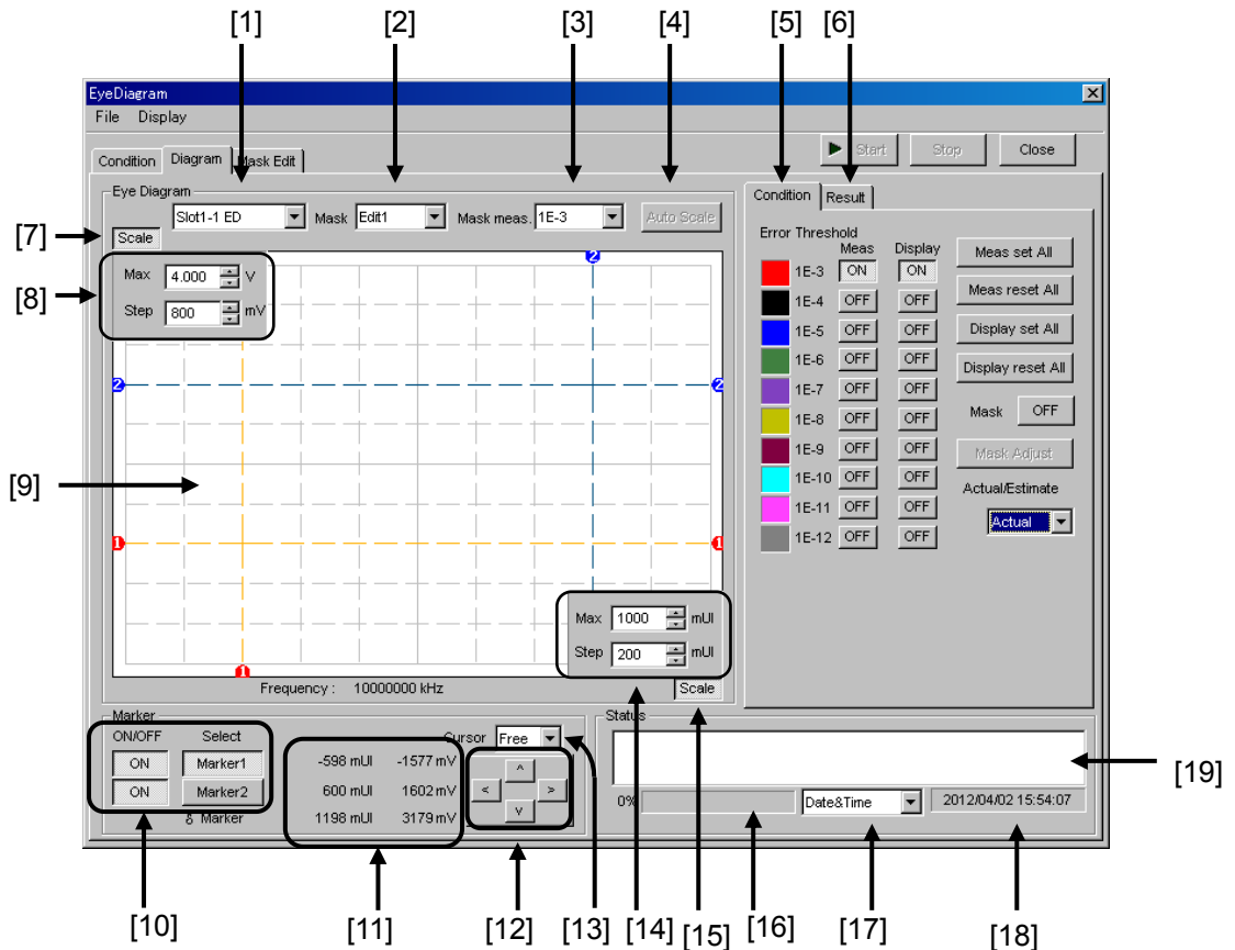
Figure 5.11.3-1 Diagram tab
