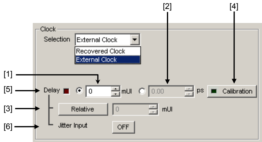
Figure 5.4.1-3 Clock Area (When External Clock Is Selected)
