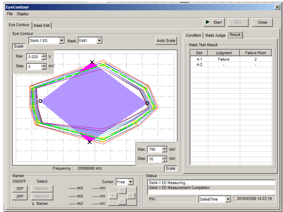
Figure 5.15.6-13 Result Tab
