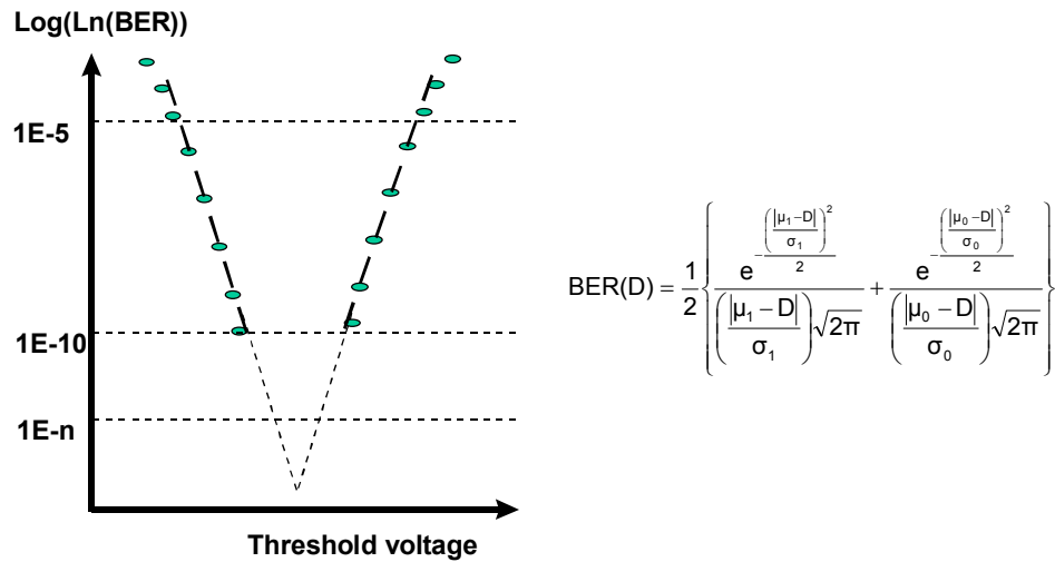
Figure 5.11.5-2 Estimated noise distribution and BER estimating expression
